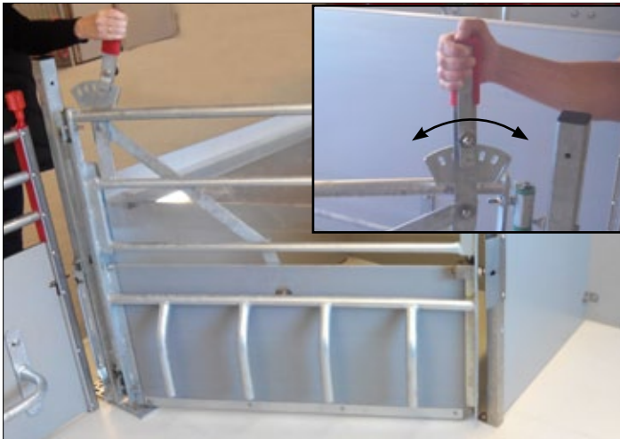
The handle is used to regulate the barrier plate's height.
